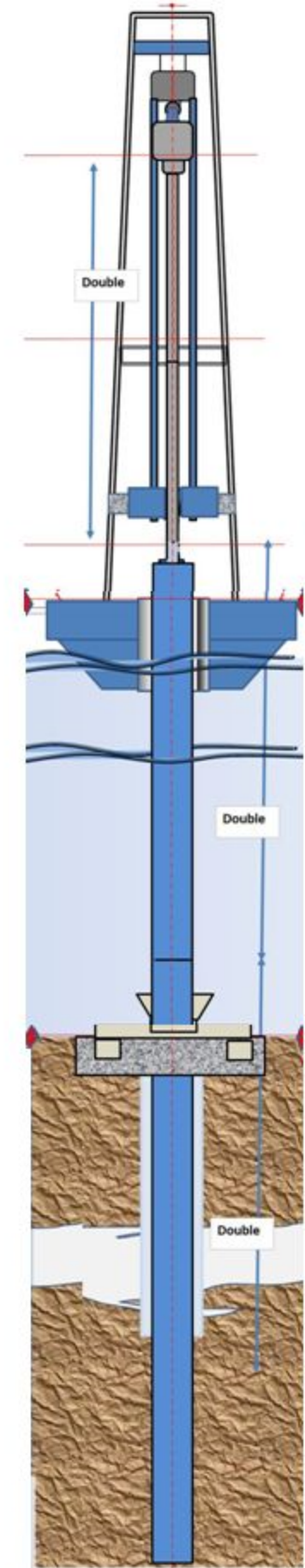
B2, Second Length of Drill Pipe Make Up and Casing Run
